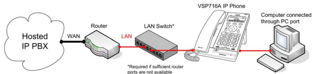
Figure 1. VSP716A Installation Example
